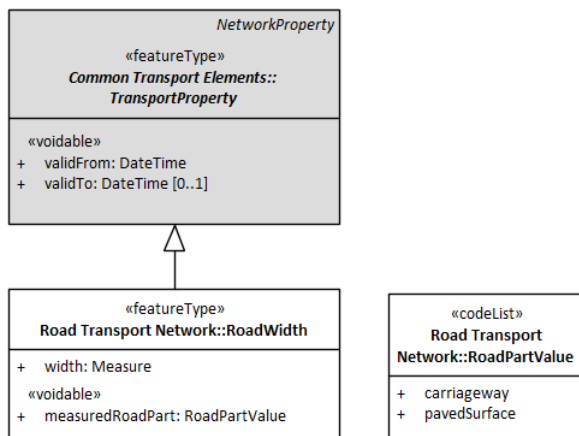
Figure 13. The INSPIRE model for road width
