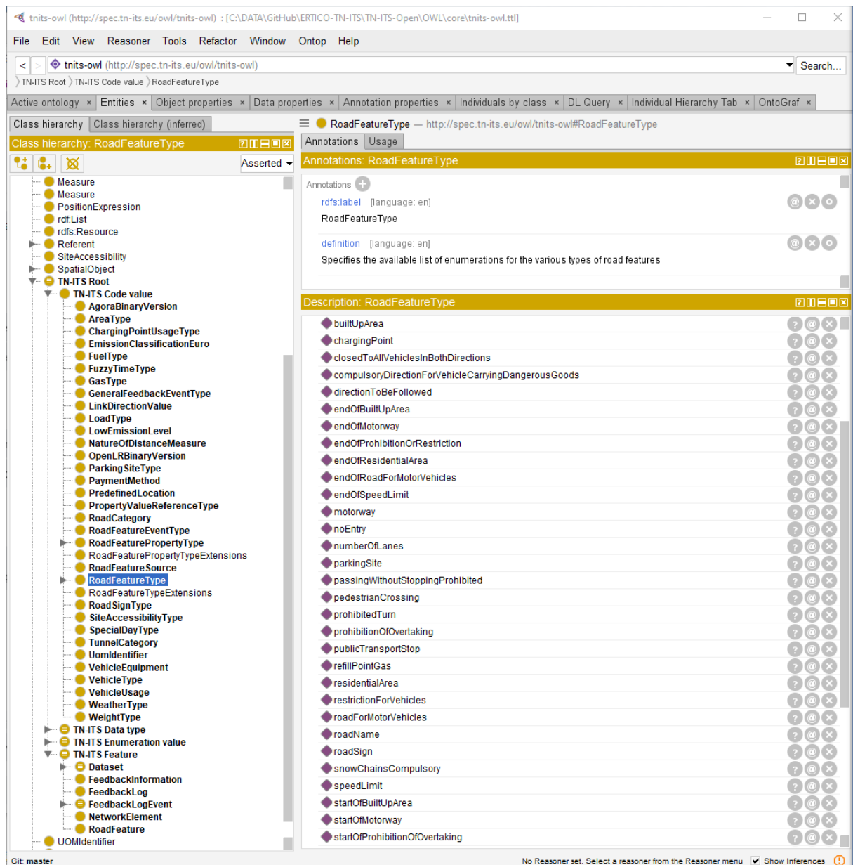
Figure 7 Some values from the TN-ITS ReadFeatureType code list. From the experimental TN-ITS Ontology .
