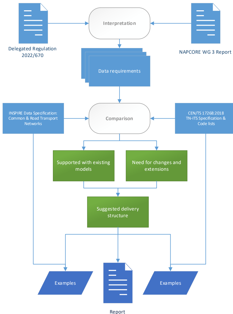
Figure 1: Methodology
