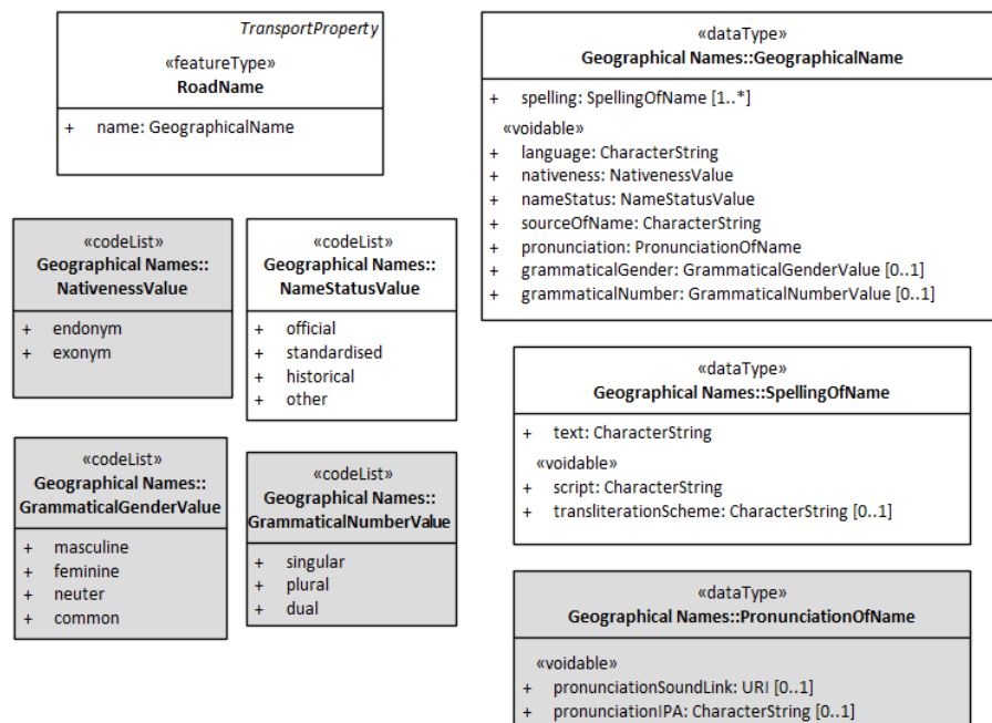
Figure 16. The INSPIRE model for geographical names
