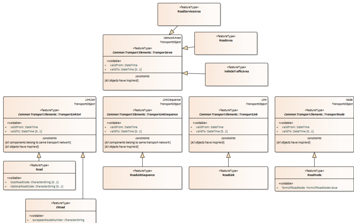
Figure 3 The Road Transport Network Model. From (INSPIRE, 2014). Original on https://inspire-mif.github.io/uml-models
