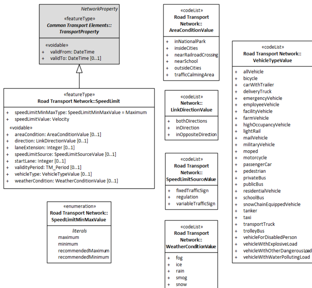
Figure 20. The INSPIRE model for speed limits
