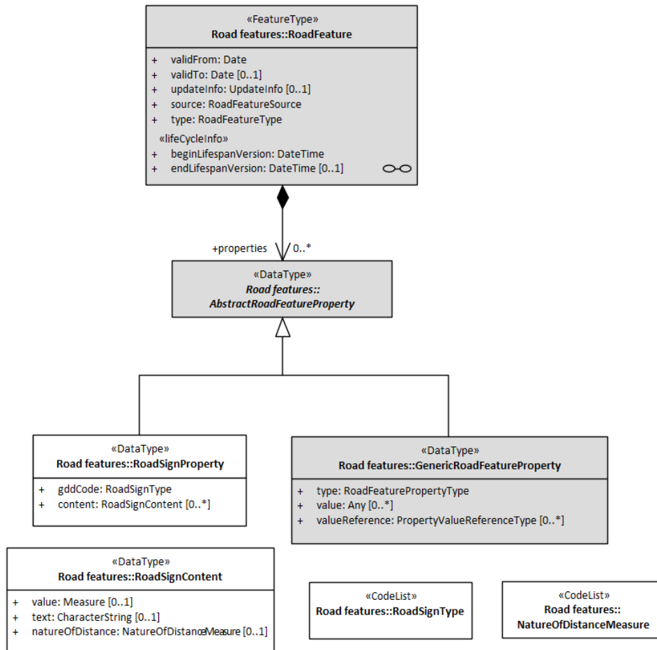
Figure 23. The TN-ITS Road sign model
