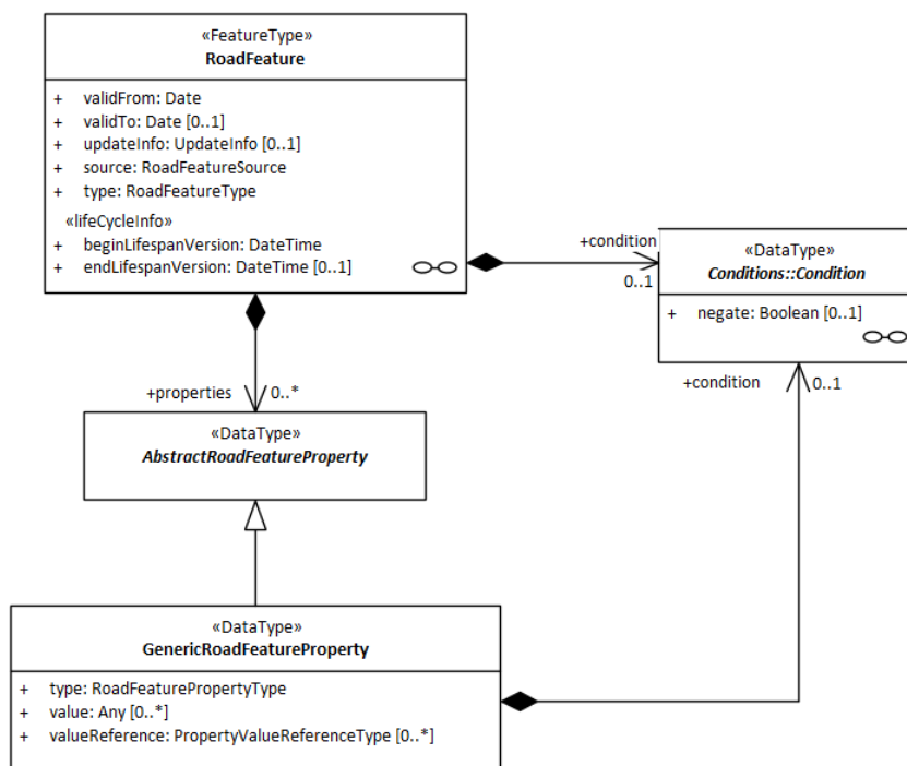
Figure 17. Conditional properties
