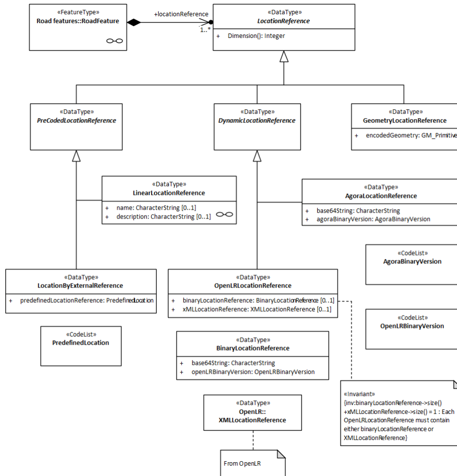
Figure 8 TN-ITS Classes for location referencing. From (CEN/TC 278, 2018)
